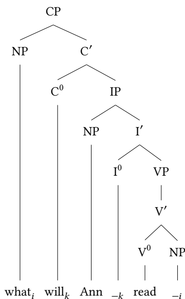
Figure 3.7: wh -question
