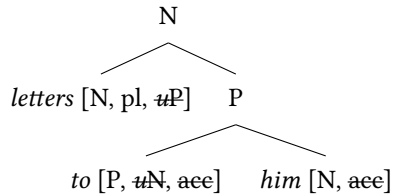
Figure 4.4: Feature checking via Agree
