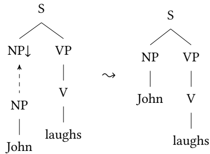
Figure 12.2: Substitution
