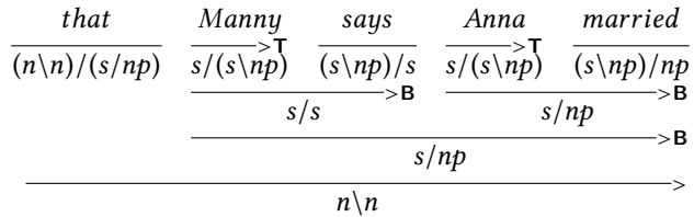
Figure 8.14: Categorial Grammar analysis of a relative clause with long-distance dependency
