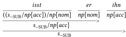
Figure 8.8: Analysis of verb-initial sentences following Steedman
