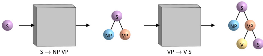
Figure 5.3: Rewrite rules and the object-transformation schema.
